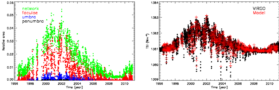
Fig. 18. The left panel gives the relative area of the full solar disk of network (green), faculae (red), umbra (blue), and penumbra (black). The right panel compares the fitted TSI data (red) with the VIRGO data corrected to the SI-scale (black).
