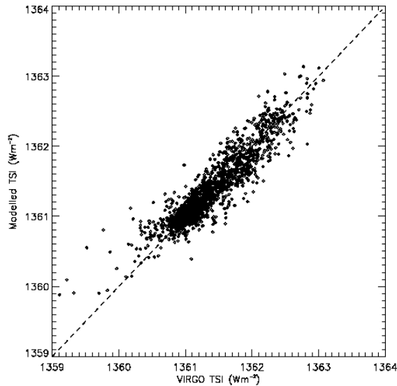
Fig. 19. Scatter plot between the VIRGO TSI data and the fitted data based on our regression analysis. The squared correlation coefficients of the fit versus the VIRGO observation is r^2 = 0.88 . The dashed line indicates equality between the two data sets.
